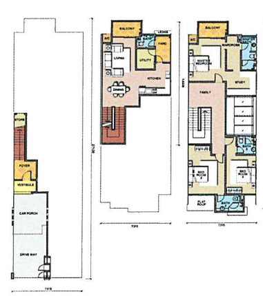
TYPE A1 24' x 90' • 2,118 sf
