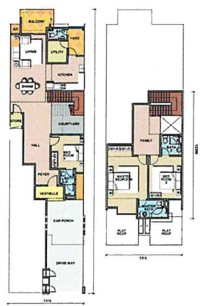
TYPE A 24' x 90' • 1,953 sf
